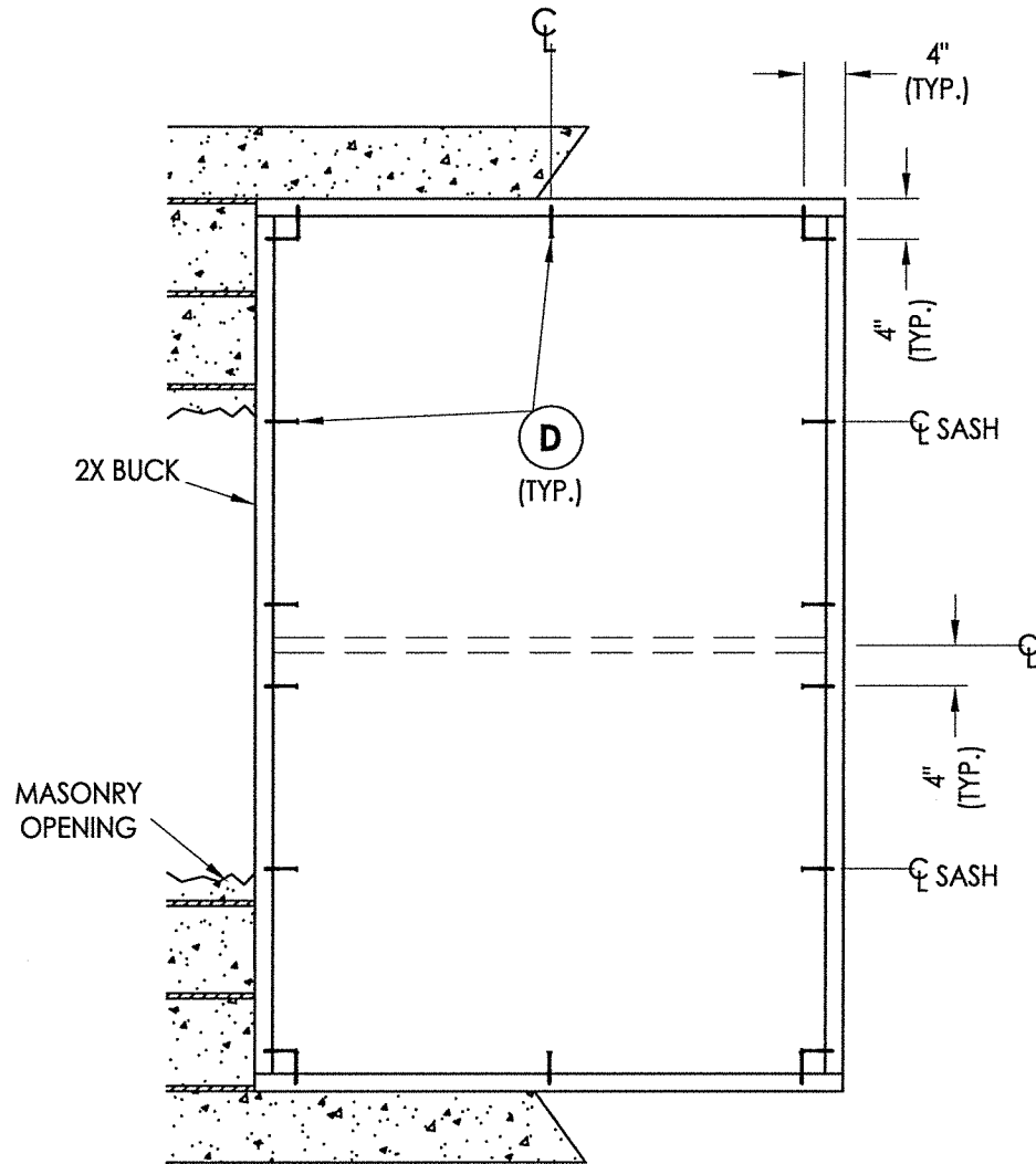
BUCK ANCHORING
