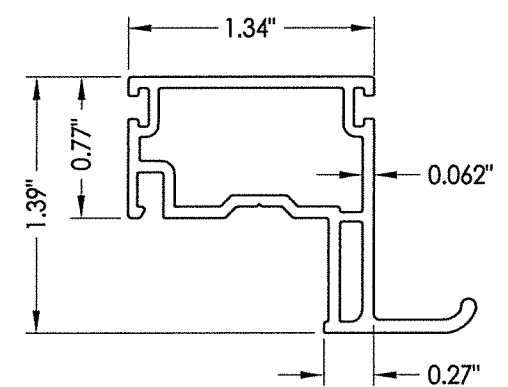
9 PULL RAIL
