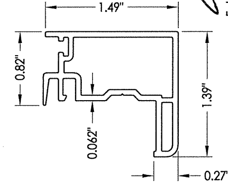
7 LOCK RAIL
