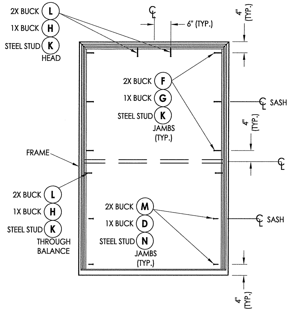
FRAME ANCHORING
