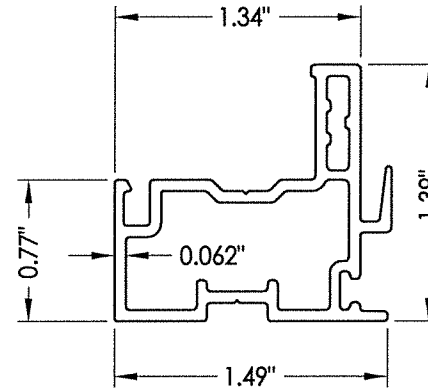
6 KEEPER RAIL
